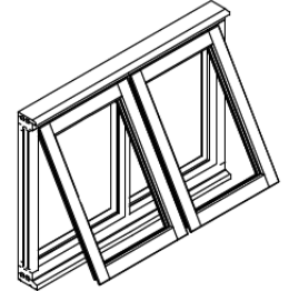
Top hinged with fixed mullion
